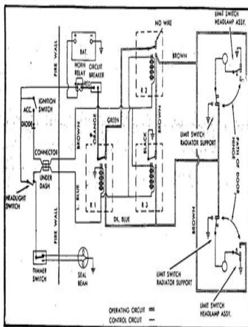
Camaro Headlamp Door Wiring-System in "Closed" Position
