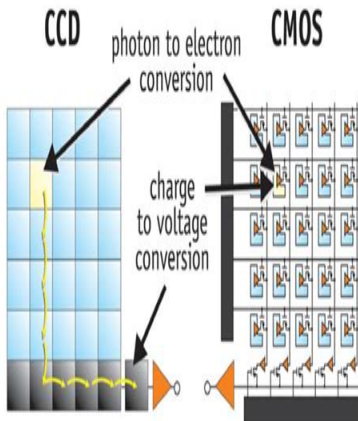
CCDs move photogenerated charge from pixel to pixel and convert it to voltage at an output node. CMOS imagers convert charge to voltage inside each pixel.
