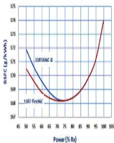
Fuel Consumption
