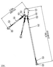
9. UPPER FRAME LIFTING JIG
